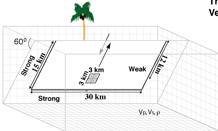
60 degree dipping Normal fault set in a homogeneous elastic halfspace
