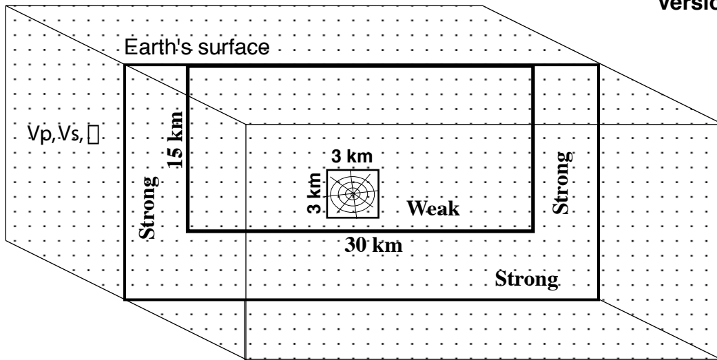
Vertical fault set in a homogeneous elastic halfspace
